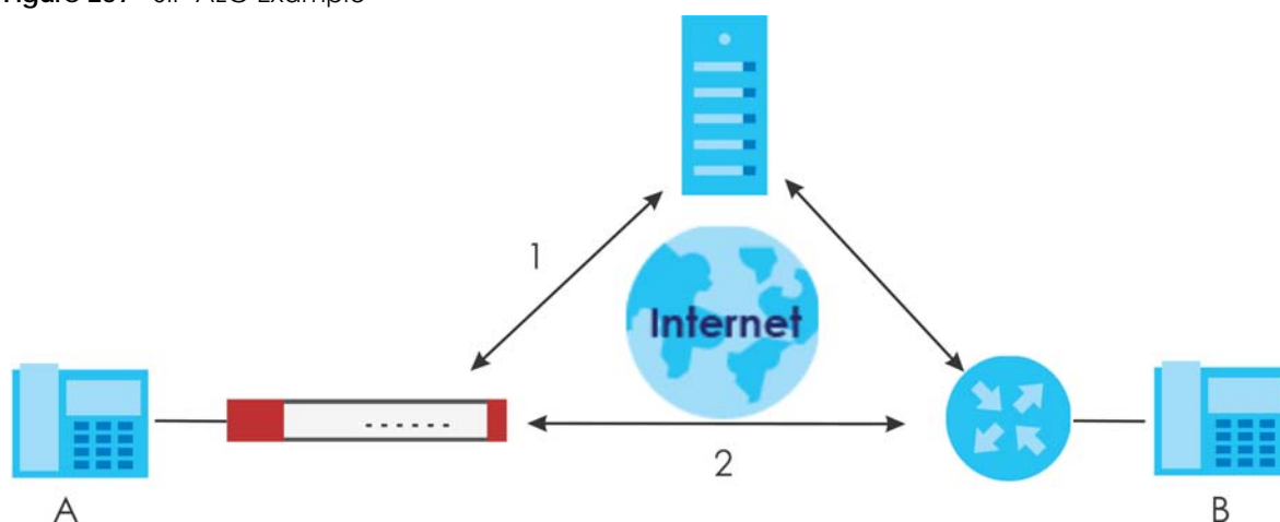
Figure 257 SIP ALG Example
